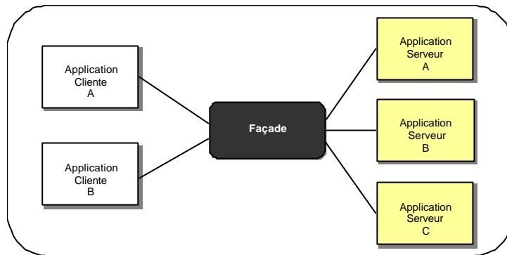
Figure III.19 Principe de la façade
